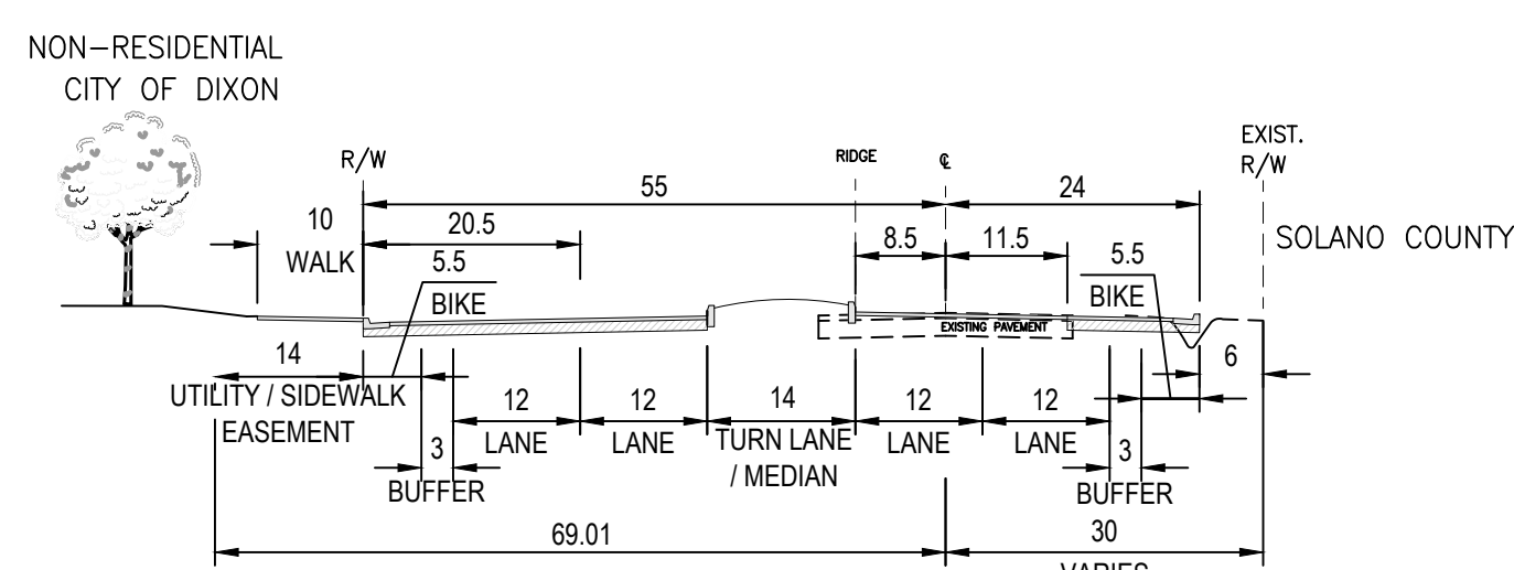
3c PEDRICK ROAD MODIFIED ARTERIAL TO EXISTING NTS
