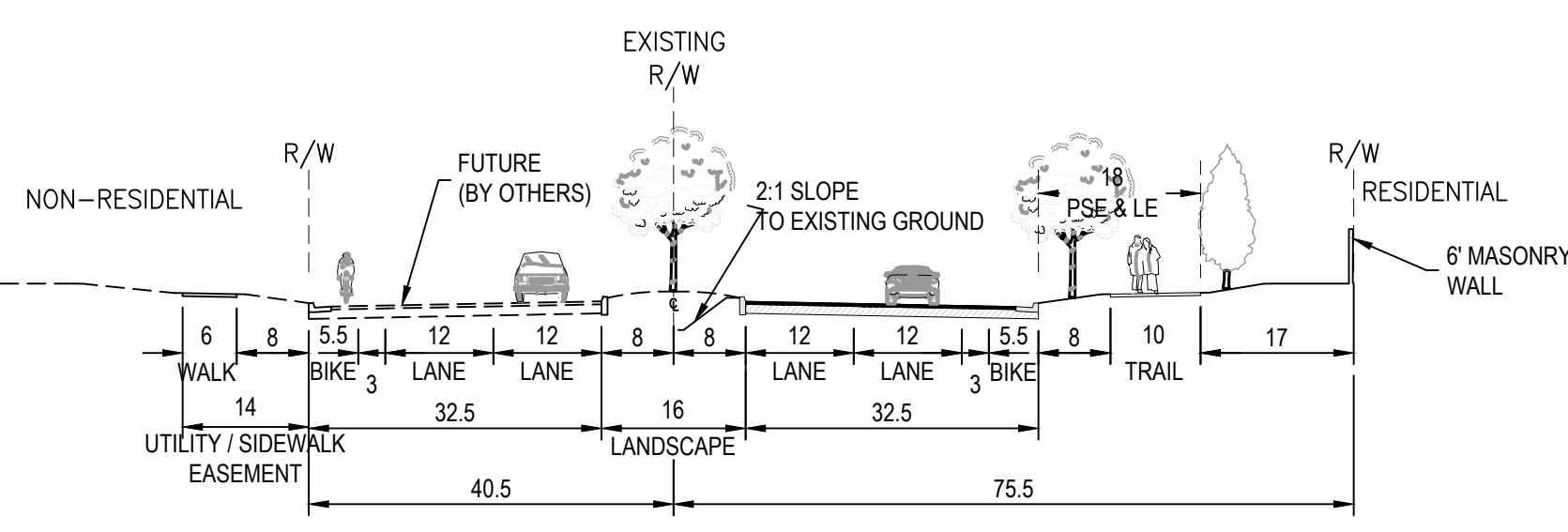
4b PROFESSIONAL DRIVE 4-LANE ARTERIAL NTS
