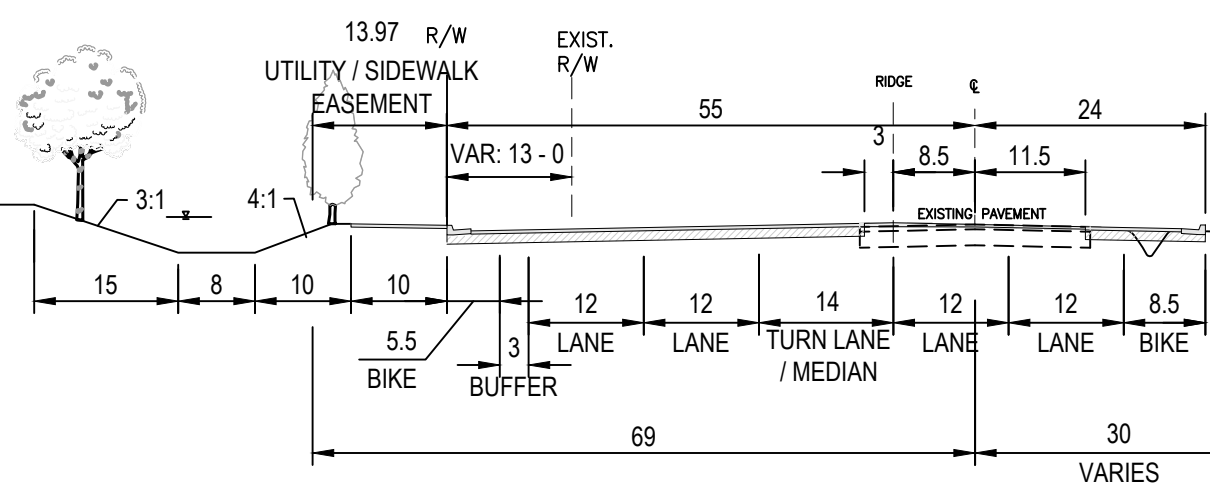
3b PEDRICK ROAD MODIFIED ARTERIAL TO EXISTING NTS
