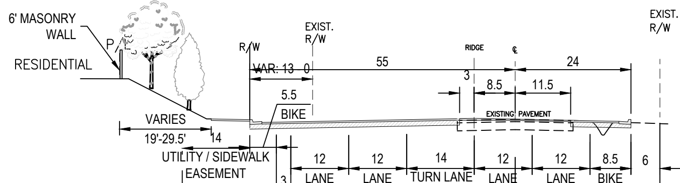
3a PEDRICK ROAD MODIFIED ARTERIAL TO EXISTING NTS
