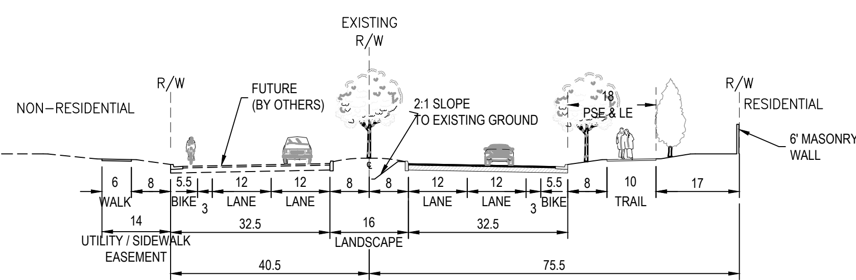
4b PROFESSIONAL DRIVE 4-LANE ARTERIAL NTS
