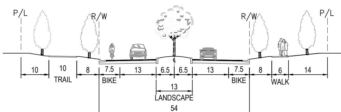
2 MAJOR COLLECTOR LANDSCAPING BOTH SIDES NTS
