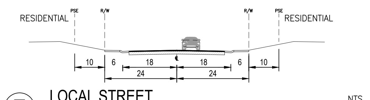
7 LOCAL STREET NTS
