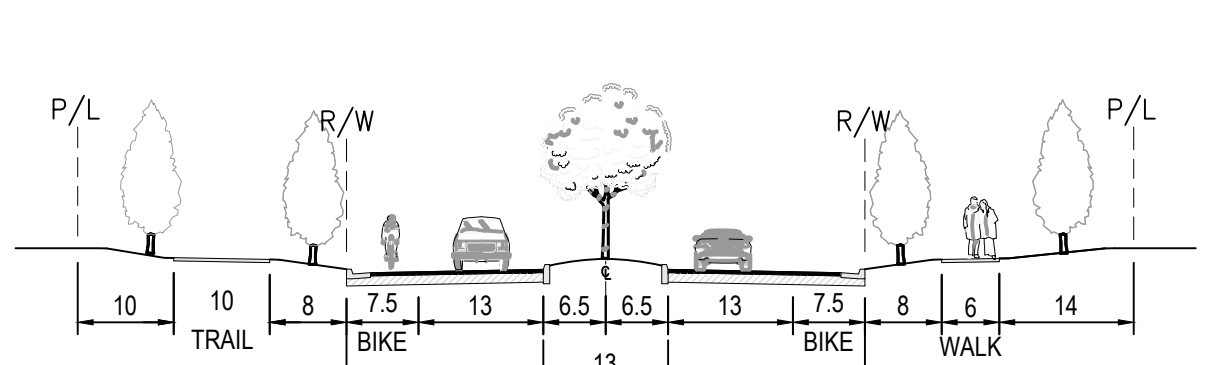
2 MAJOR COLLECTOR LANDSCAPING BOTH SIDES NTS
