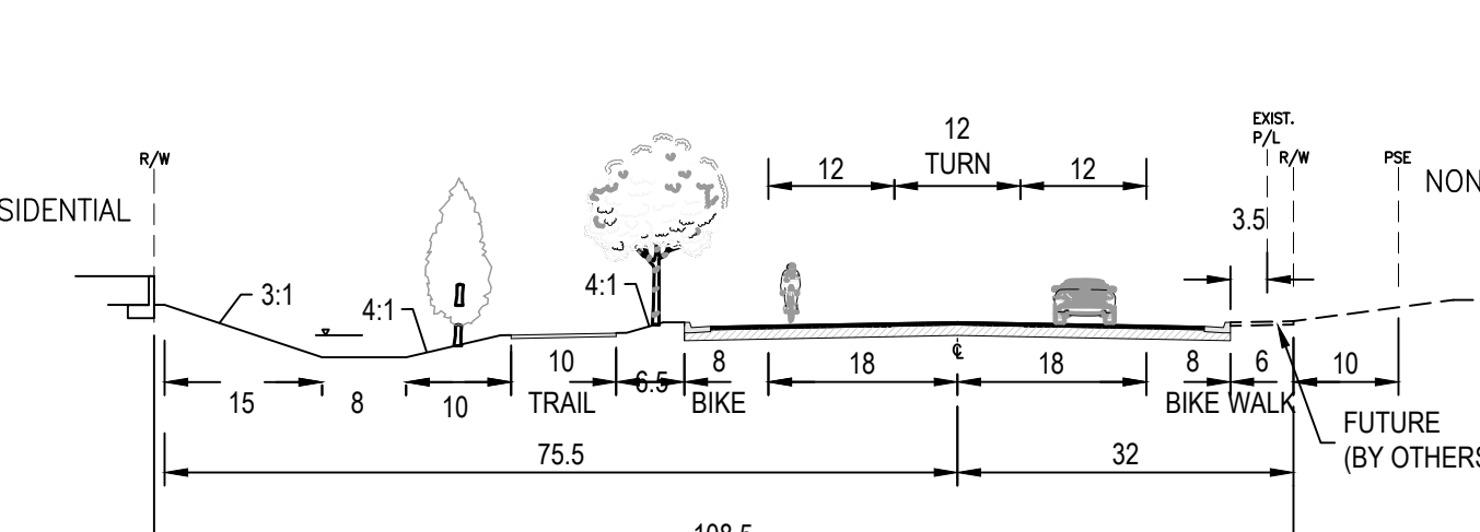
5 COMMERCIAL DRIVE COLLECTOR ROADWAY NTS
