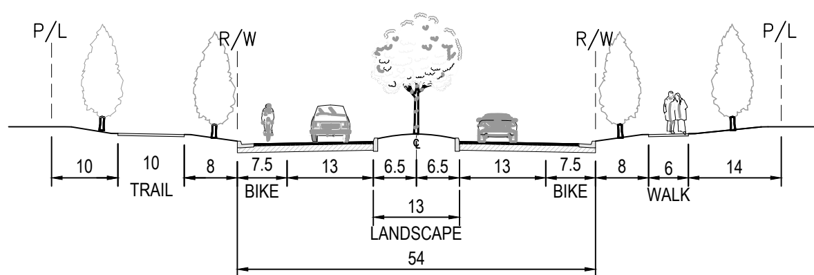
2 MAJOR COLLECTOR LANDSCAPING BOTH SIDES NTS
