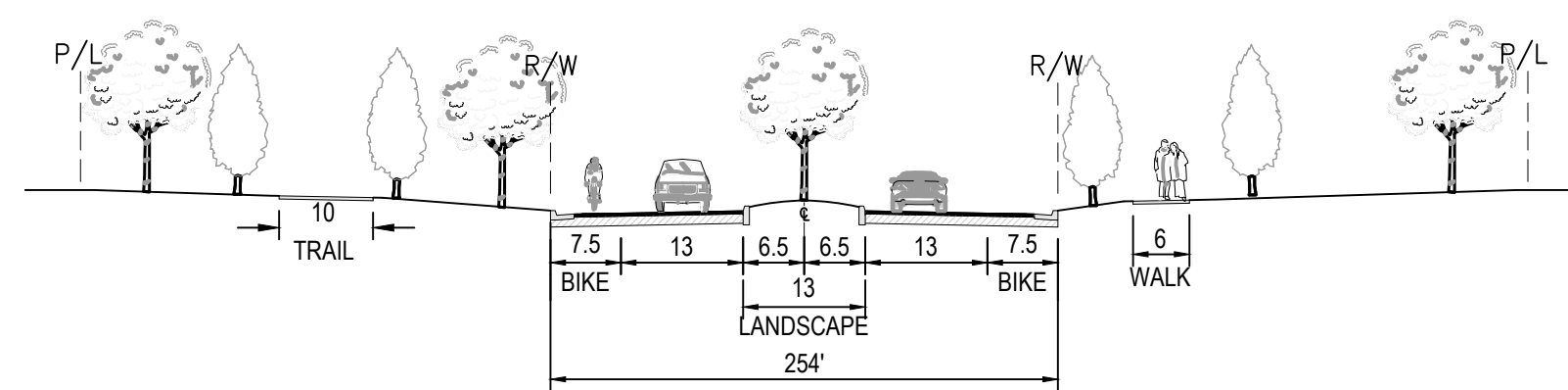
1 MAJOR COLLECTOR ADJACENT TO LINEAR PARK NTS
